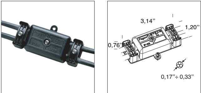
Cable connector IP68 4 ways - series connection
