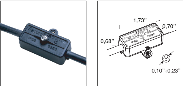
Cable connector IP68 2 ways - direct connection
