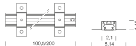
WALL MOUNTED
