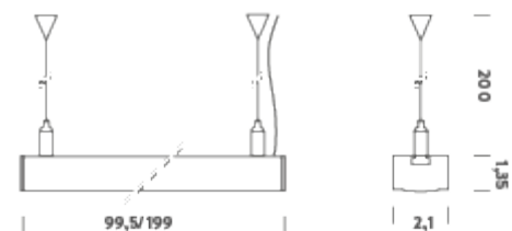
CEILING
