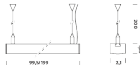
CEILING
