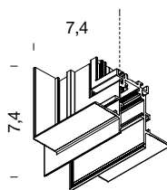
TRIMLESS TRACK WALL CORNER EXTERNAL
