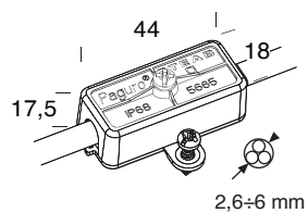
BCONN2IP68 Cable connector IP68 2 ways (not included/external)
