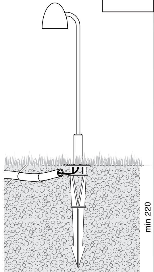
Bottom cable exit
